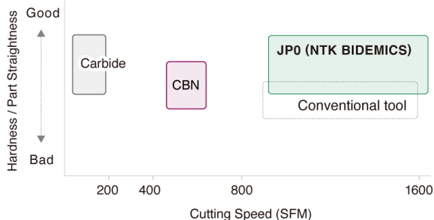
JP0 - Machine with a consistent DOC to provide stable tool life
