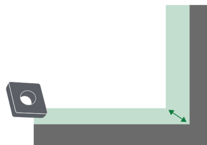
JP0 - Machine with a consistent DOC to provide stable tool life
