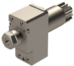
MSC-507-2X Cross Drill/Mill Collet Size: ER11 Output: 1:2 High Speed
