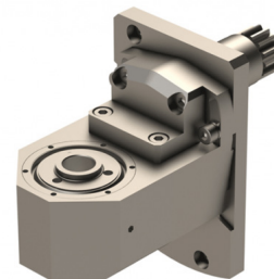
LSW-515 Thread Whirling Ring: Utilis Output: 1:1 7 or 9 Insert Cutter Flight Circle: Ø6mm
