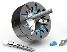
Thread Whirling
